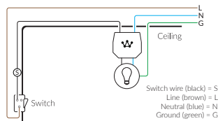
B) Crownstone is placed at the ceiling.
