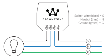
C) Built-in Crownstone connection diagram. Wire colors may be different in your situation.
