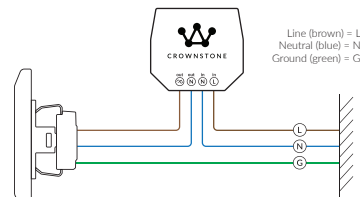
A) Built-in Crownstone connection diagram. Wire colors may be different in your socket.
